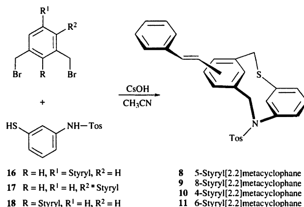
Scheme 4 Synthesis of tosylated [2.2]metacyclophanes with stilbene units 8–11
