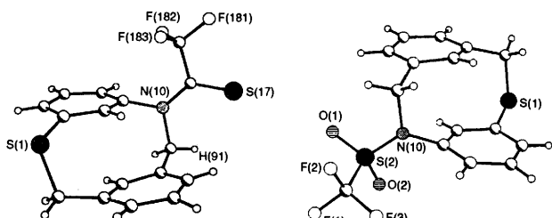
Fig. 1 X-Ray structures of the N -substituted cyclophanes 3 and 4
