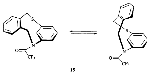
Scheme 3 synlanti Conformational process for the N -trifluoroacetyl-1-thia-10-aza[2.2]orthometacyclophane 15
