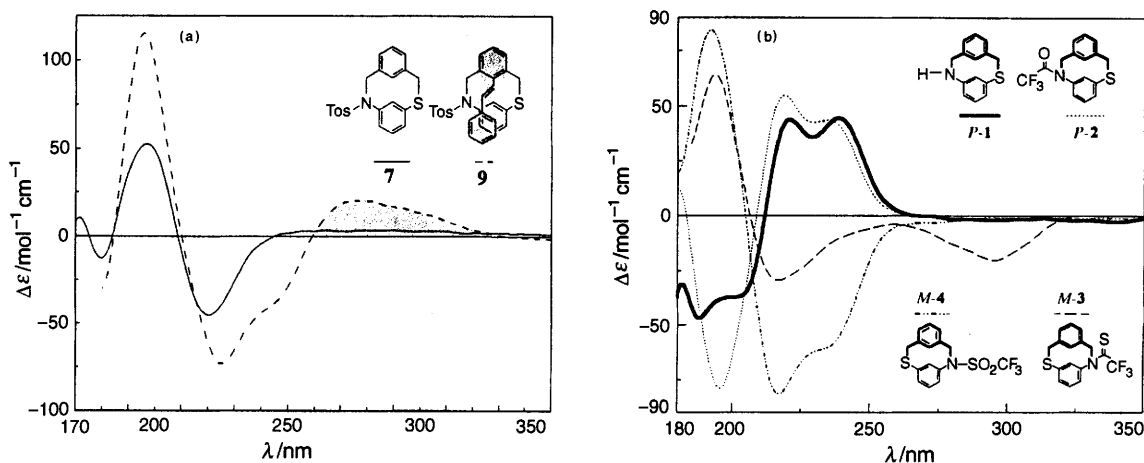
Fig. 2 (a) CD spectra of the stilbenophane 9 , compared to the unsubstituted compound 7 ; solvent hexafluoropropan-2-ol; (b) CD spectra of the different N -derivatives; solvent hexafluoropropan-2-ol; P-1 (—), P-2 (····), M-3 (---), M-4 (-·-·-)
